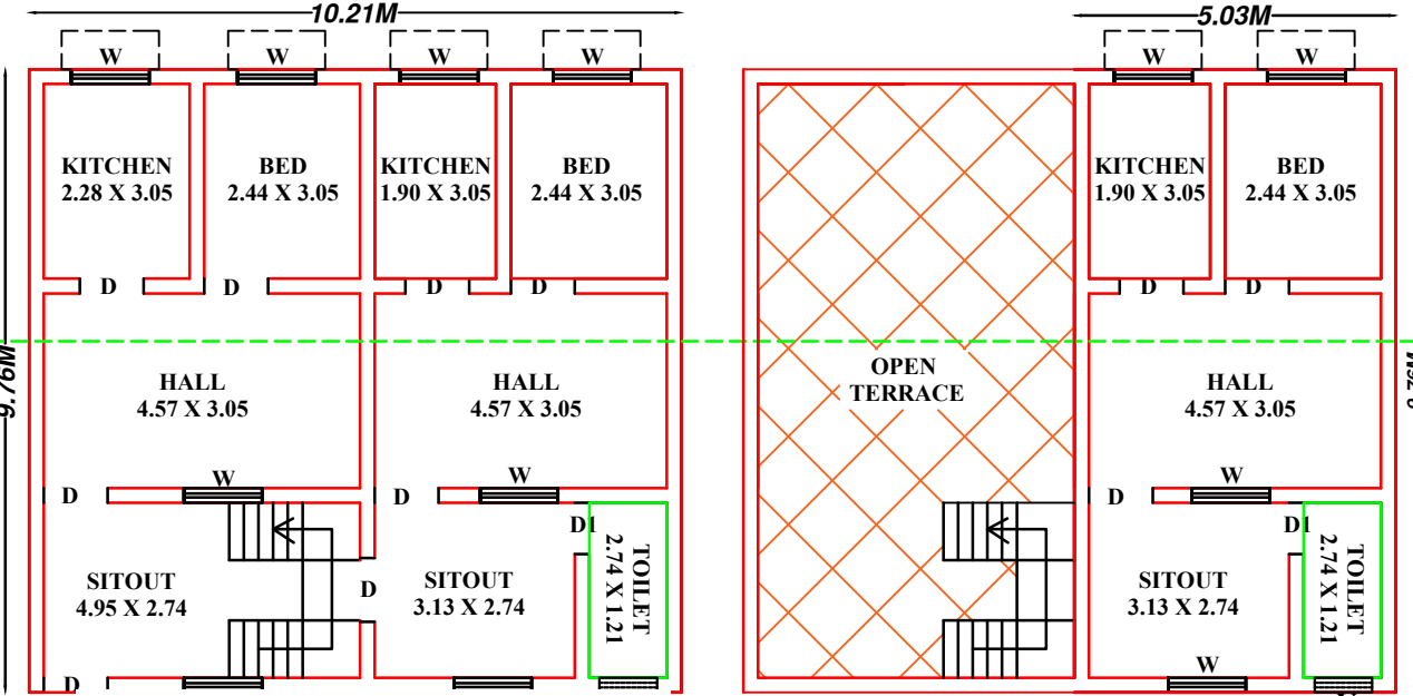
PRO.ADD FIRST FLOOR PLAN
