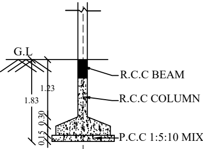
SECTION OF FOOTING
