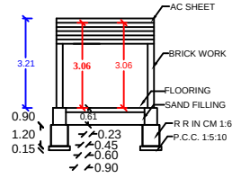
SECTION AB
