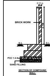
SECTION OF COMPOUND WALL
