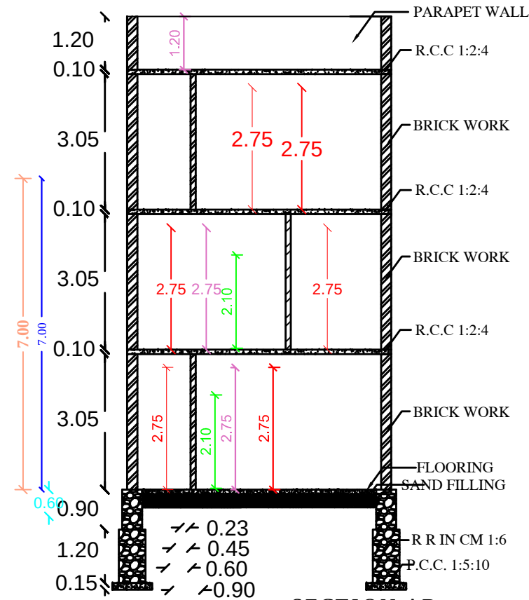
SECTION AB
