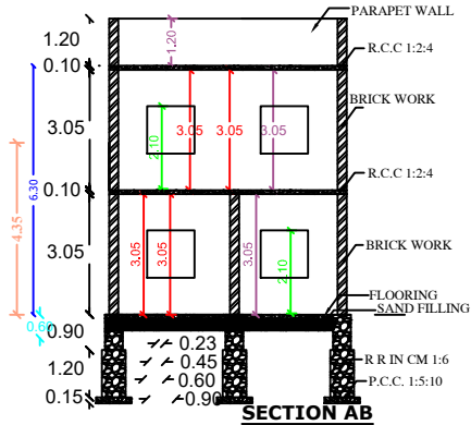
SECTION AB
