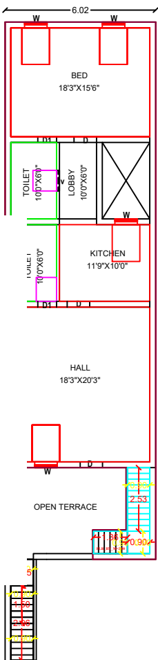
PRO.FIRST FLOOR PLAN
