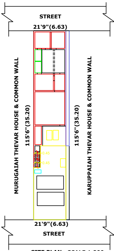
SITE PLAN SCALE 1:200
