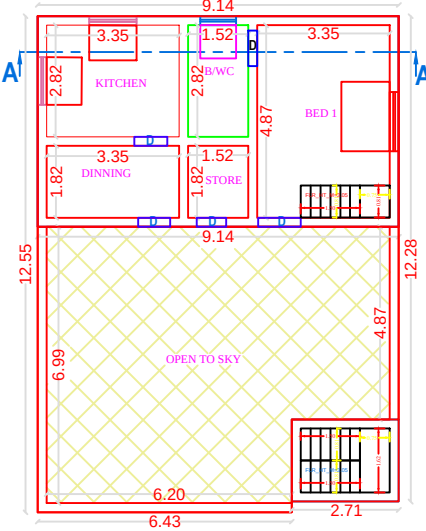
PLAN - FIRST FLOOR (PROPOSED)
