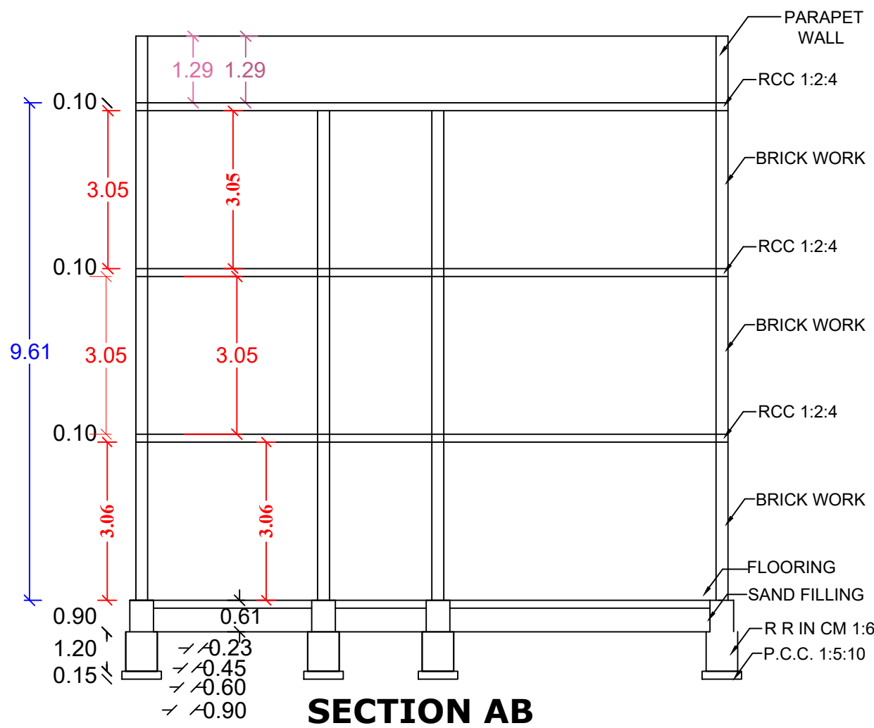
SECTION AB
