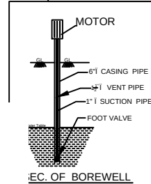
SECTION OF BOREWELL
