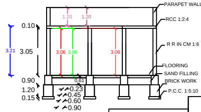
SECTION AB
