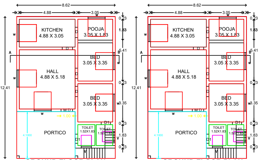
GROUND FLOOR PLAN HOUSE - 1
