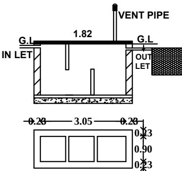
SEPTICTANK DETAILS
