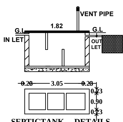
SEPTICTANK DETAILS
