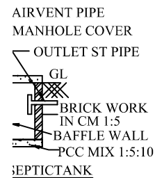
SEPTICTANK
