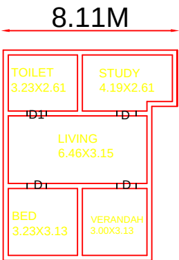
EXISTING BUILDING PLAN
