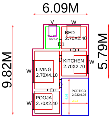
PROPOSED BUILDING PLAN
