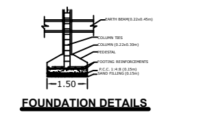
FOUNDATION DETAILS
