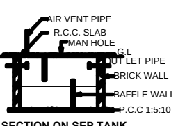
SECTION ON SEP.TANK
