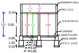
SECTION AB
