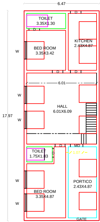
PROPOSED GF PLAN
