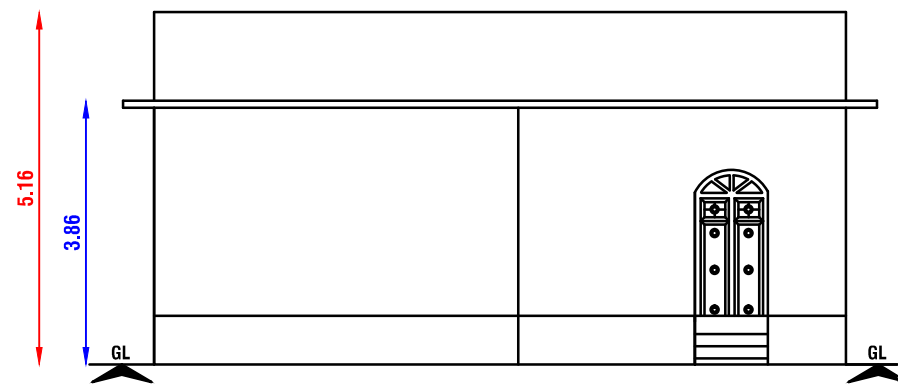
FRONT ELEVATION
