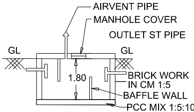
SECTION ON SEPTICTANK
