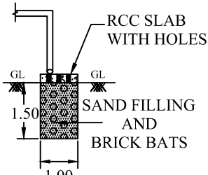
SECTION OF BS
