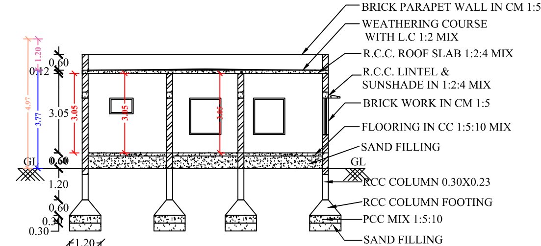
SECTION OF "AB"
