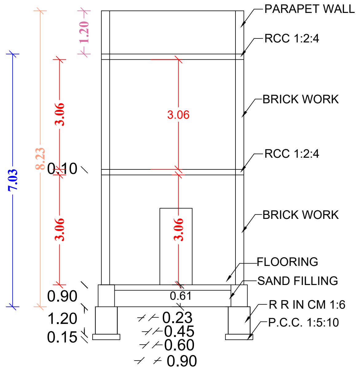
SECTION AB
