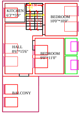
PROPOSED F.FLOOR PLAN
