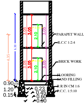
SECTION AB
