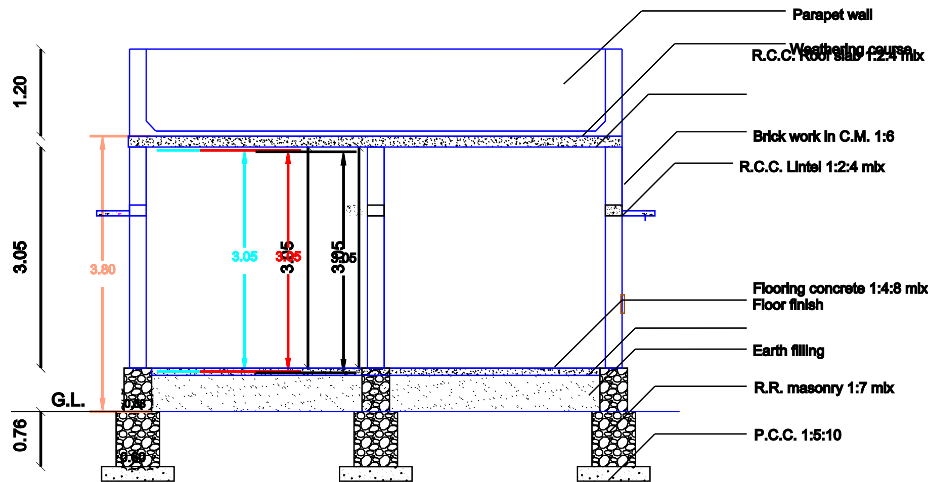
SECTION AB
