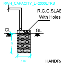
SECTION ON 'AB'
