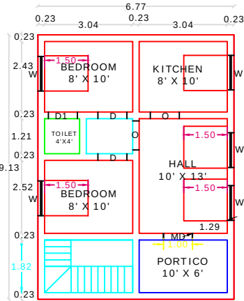
GROUND FLOOR RESIDENTIAL PLAN
