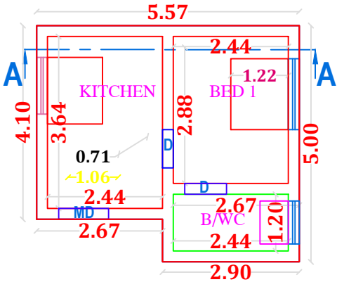
PLAN - GROUND FLOOR (PROPOSED)
