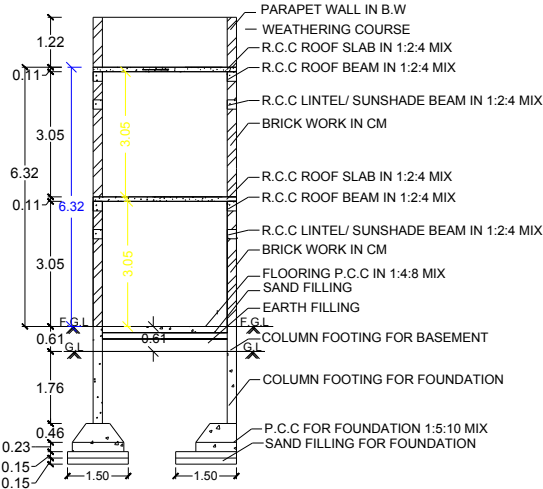
SECTION ON-AA
