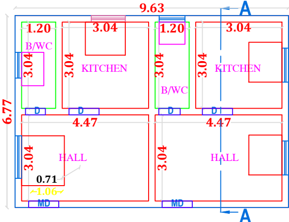
PLAN - GROUND FLOOR (PROPOSED)
