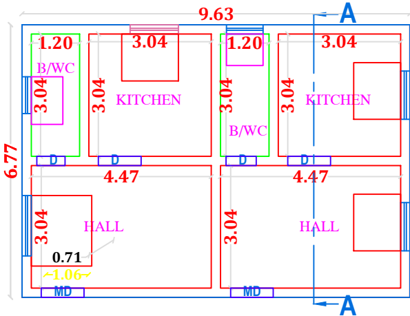
PLAN - GROUND FLOOR (PROPOSED)
