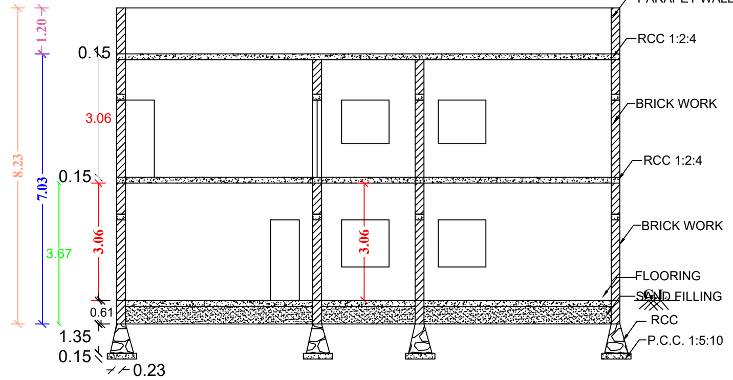
SECTION AB
