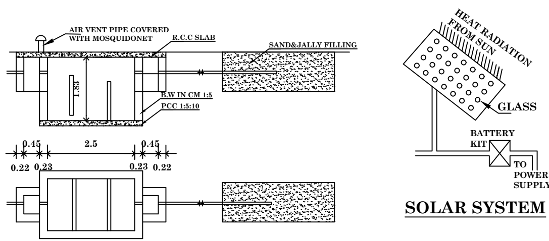
PLAN&SECTION OF SEPTIC TANK TRENCH
