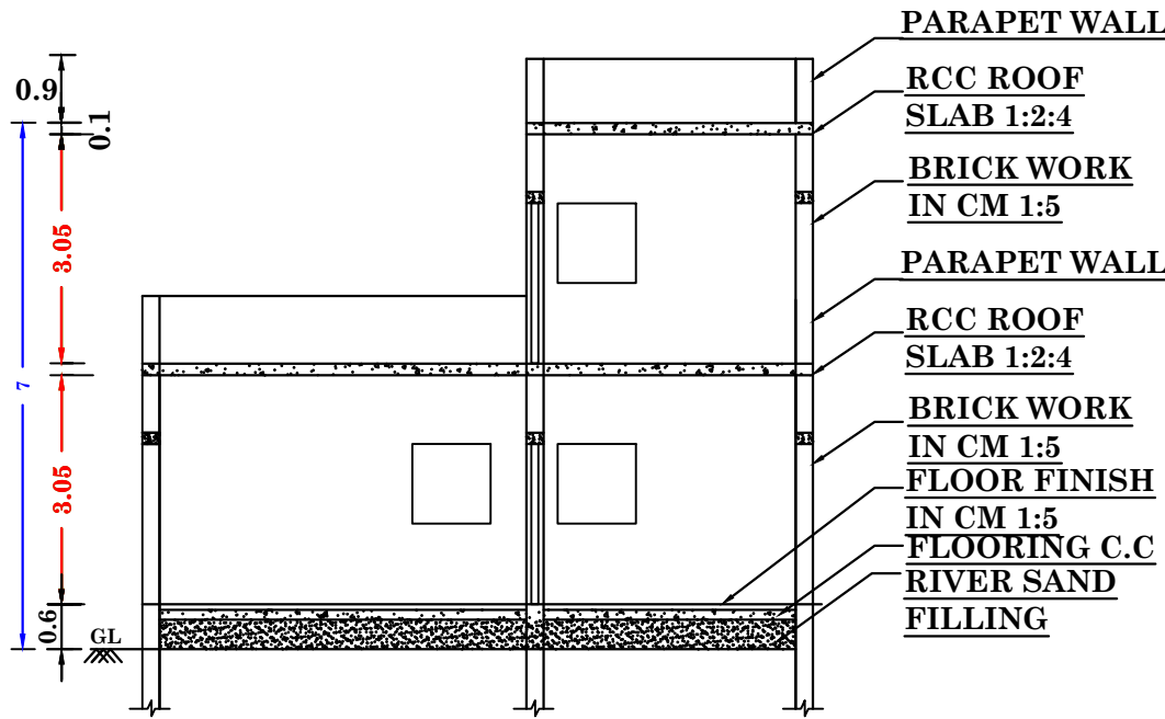
SECTION ON AA1
