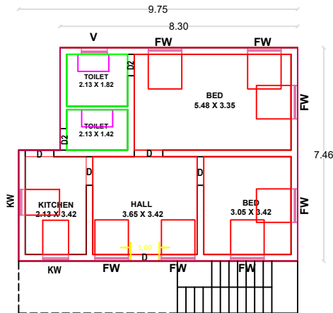
PLAN - GROUND FLOOR (PROPOSED)
