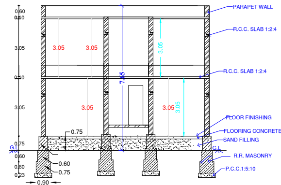
SECTION AB
