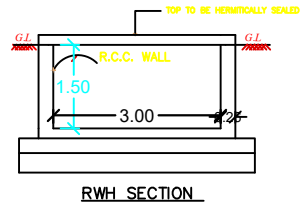
RWH SECTION
