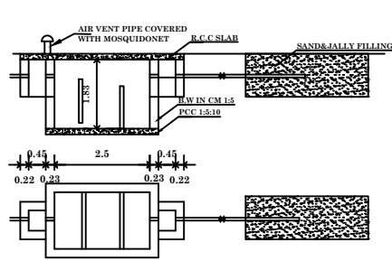
PLAN&SECTION OF SEPTIC TANK TRENCH
