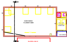
BLOCK-1 GROUND FLOOR PLAN TYPICAL_FLOOR_PLAN=1
