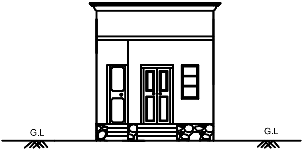
FRONT ELEVATION
