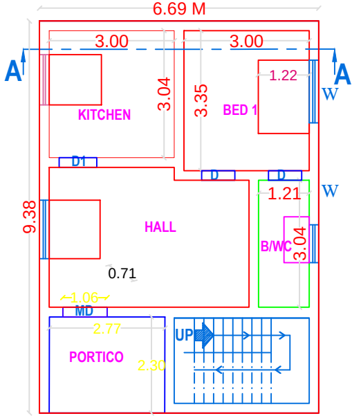
PLAN - GROUND FLOOR ( PROPOSED )
