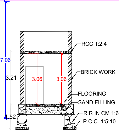
SECTION ON A - B
