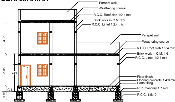
SECTION AB
