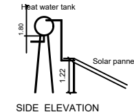
SIDE ELEVATION
