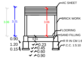
SECTION AB
