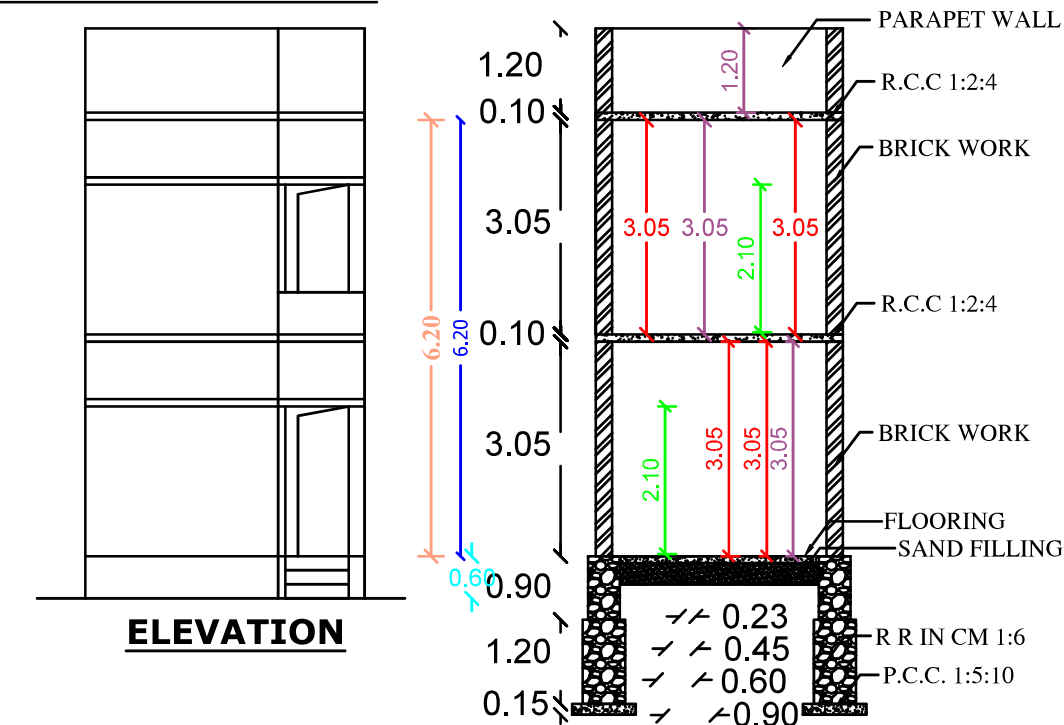
SECTION AB
