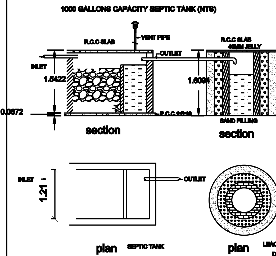
plan SEPTIC TANK
