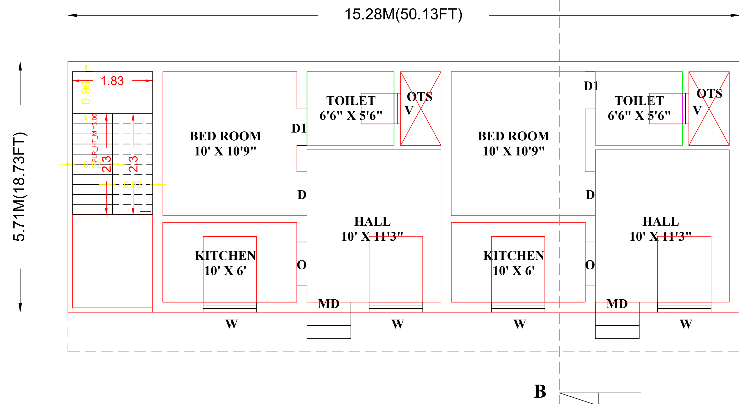
EXTG.GROUND FLOOR PLAN
