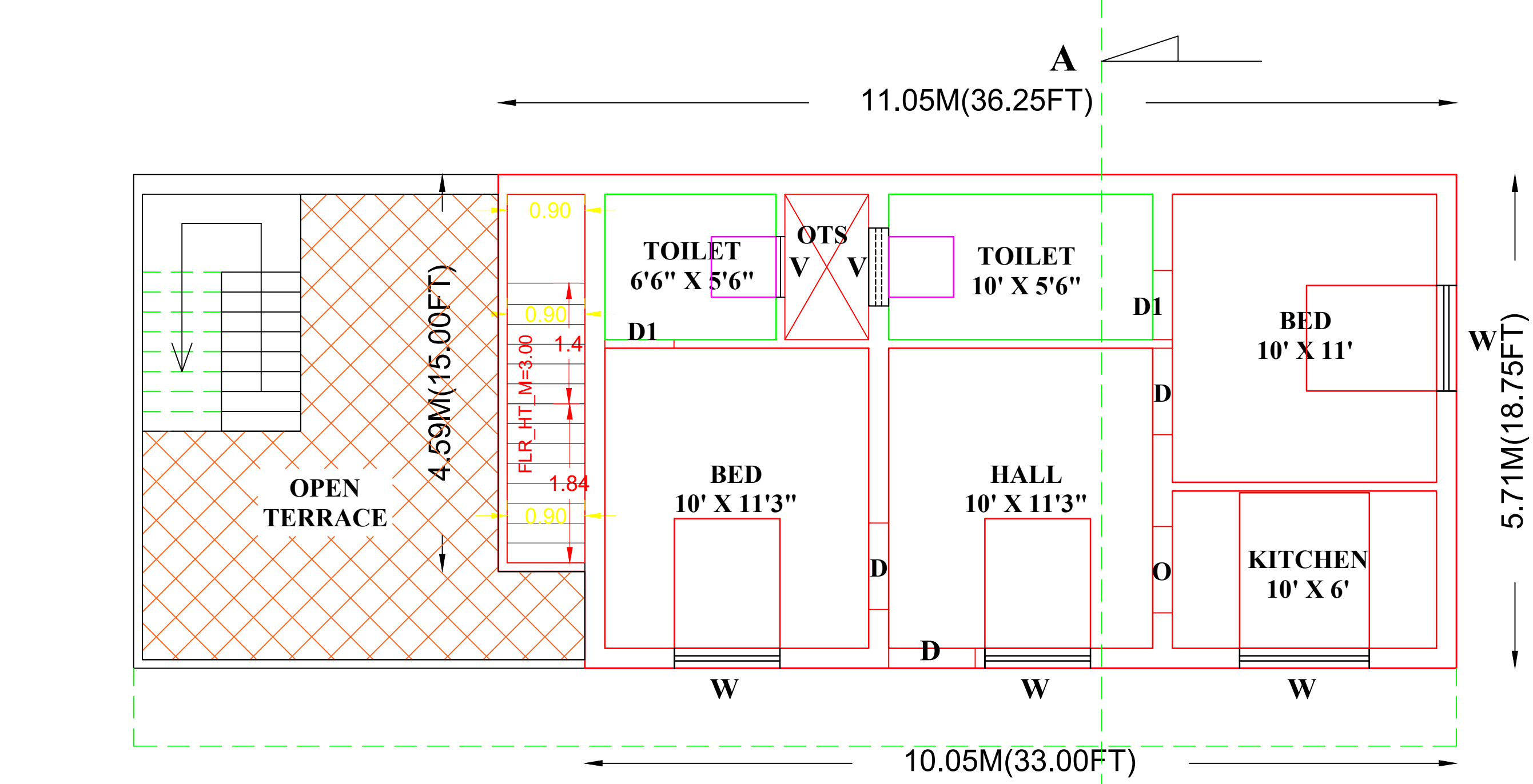
PRO.FIRST FLOOR PLAN
