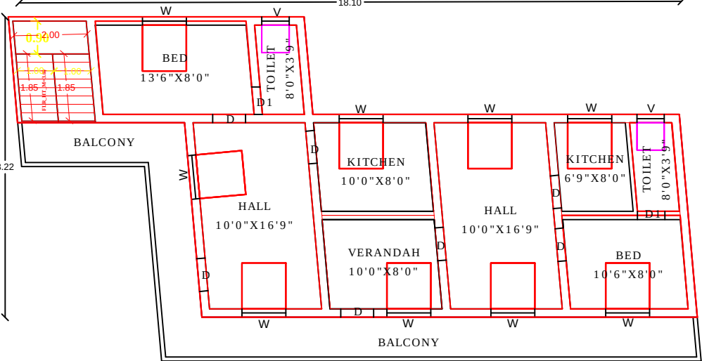
PRO.FIRST FLOOR PLAN
