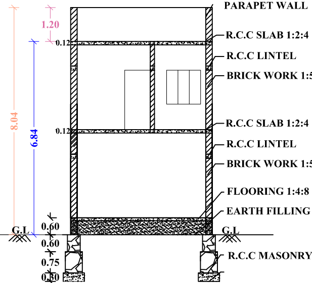
"SECTION 'AB'"
