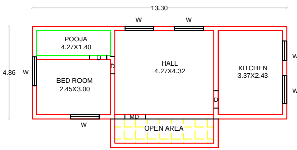
PROPOSED FF PLAN
