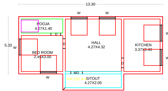
PROPOSED GF PLAN
