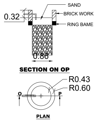
RAIN WATER PIT
