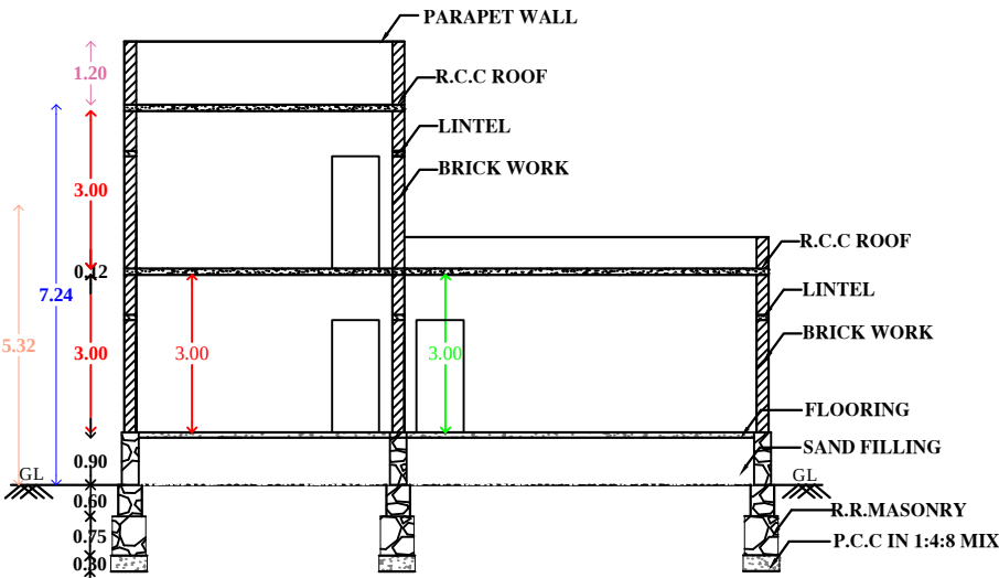
"SECTION "AB"
