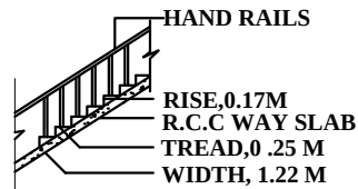
SECTION ON STAIR
