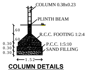
COLUMN DETAILS
