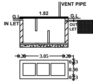
SEPTICTANK DETAILS
