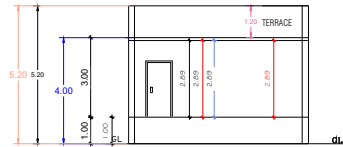
SECTION "A-A" (PROPOSED)
