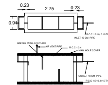
SECTION OF RAINWATER COLLECTING TANK
