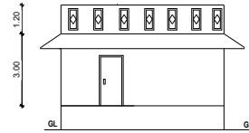
ELEVATION (PROPOSED)
