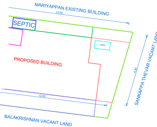
SITE PLAN
