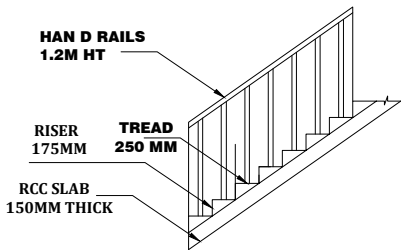
STAIRCASE DETAILS SCALE 1:50
