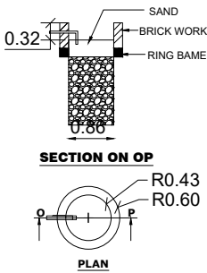
RAIN WATER PIT
