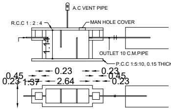
SEPTIC TANK & TRENCH
